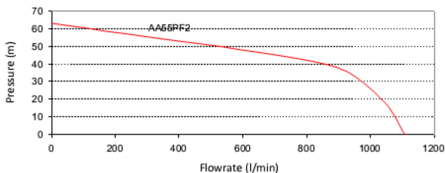
Flow curve for AA55 PF2 pump
